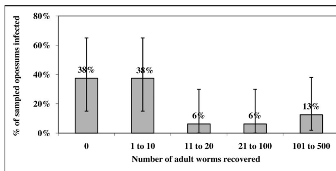
FIGURE 2. Cruzia americana adult worm burdens from intestinal washes and feces from opossums sampled in Monterey and Rio Vista, California. Exact binomial 95% confidence intervals are from Epi Info™ version 3.3.2 (CDC, Atlanta, Georgia).
